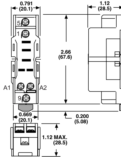
Figure 5: 781-1C-SKT Dimensions
