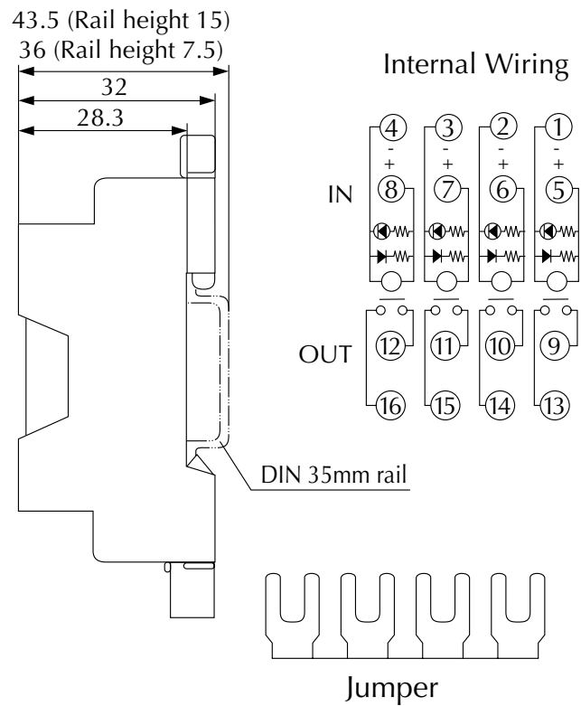
Wiring diagram RS6N-DE
